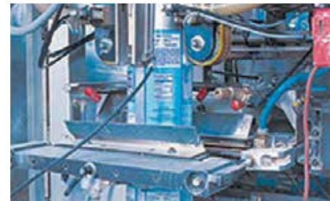
Plastic bags seamed and sealed by VFFS machinery
